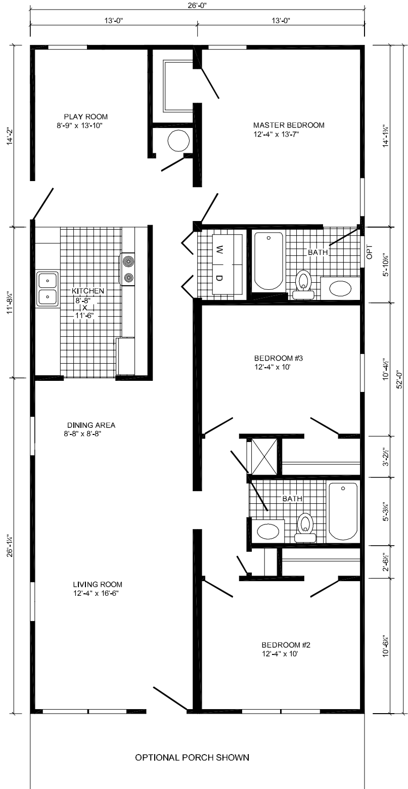
OPTIONAL PORCH SHOWN. STAIRS, RAILS, ETC. ON SITE BY OTHERS
